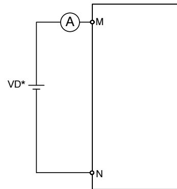
Figure 12. Test Circuit for I_D
