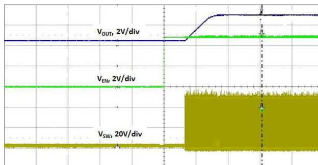
Fig. 7 - Pre-Bias Start-Up
