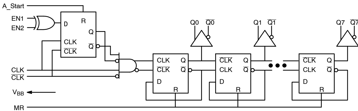
Figure 2. Logic Diagram
