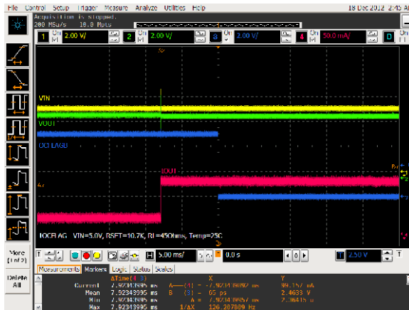
Figure 9. OC_FLAGB Response Time (Toggle R_{LOAD} from High to Low Resistance)
