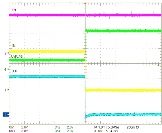
Figure 6. Power-Down Transient ( V_{IN} = 5V , C_{OUT} = 0.1\mu F )
