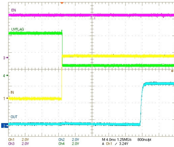
Figure 5. Power-Up Transient ( V_{IN} = 5V , C_{OUT} = 0.1\mu F )
